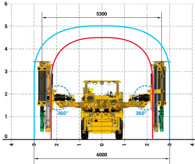
Transverse Coverage
