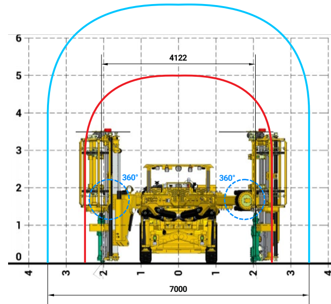
Transverse Coverage
