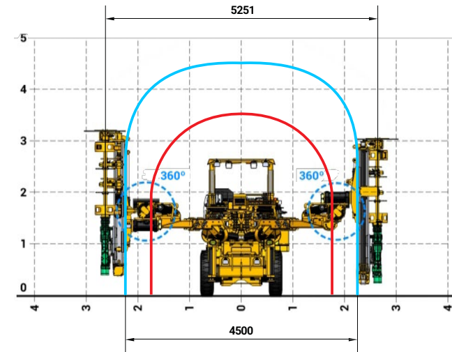
Transverse Coverage
