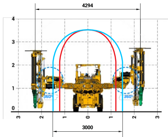
Transverse Coverage
